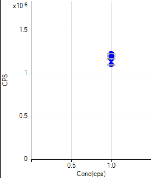
89 Y(ISTD) [He]
