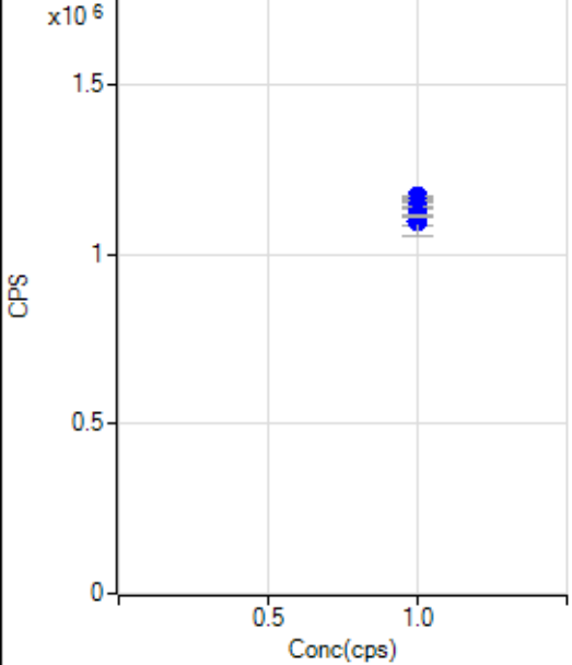
89 Y(ISTD) [He]
