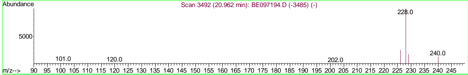
TIC: BE097208.D
