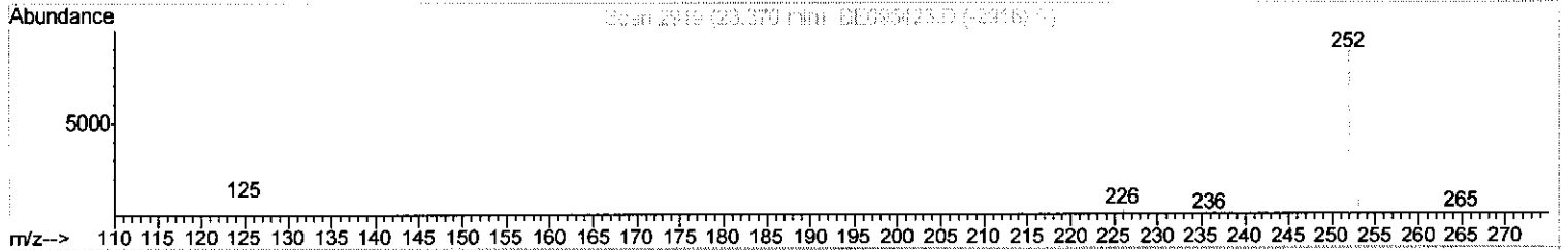
TIC: BE095430.D
