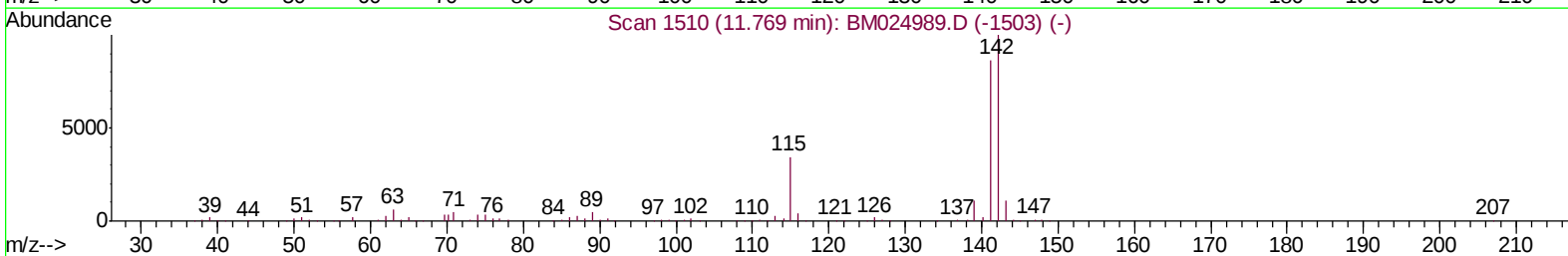
TIC: BM024998.D
