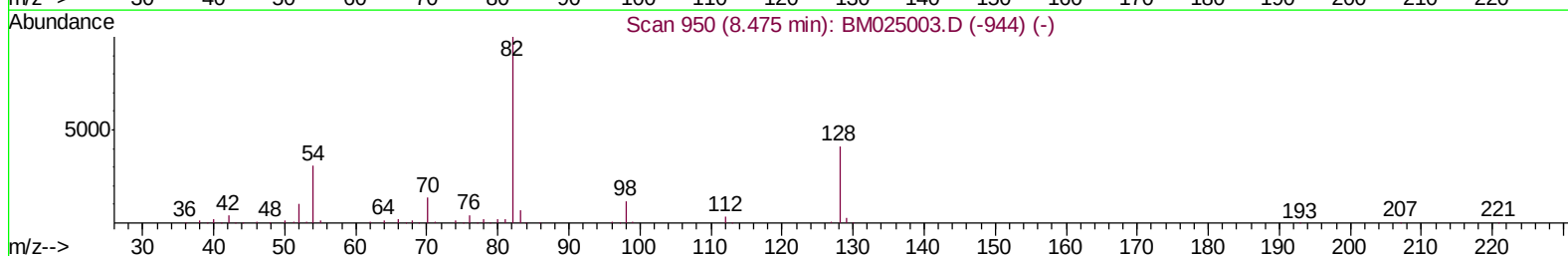
TIC: BM025015.D
