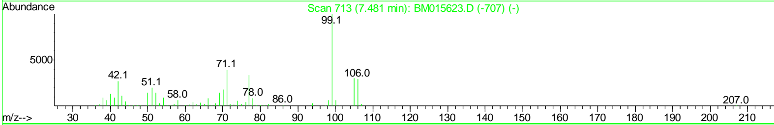
TIC: BM015630.D
