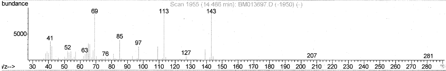
TIC: BM013716.D
