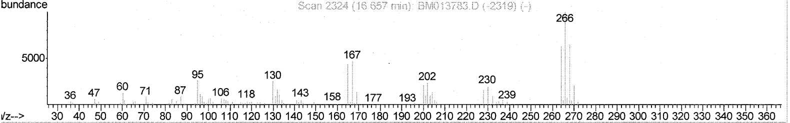
TIC: BM013799.D
