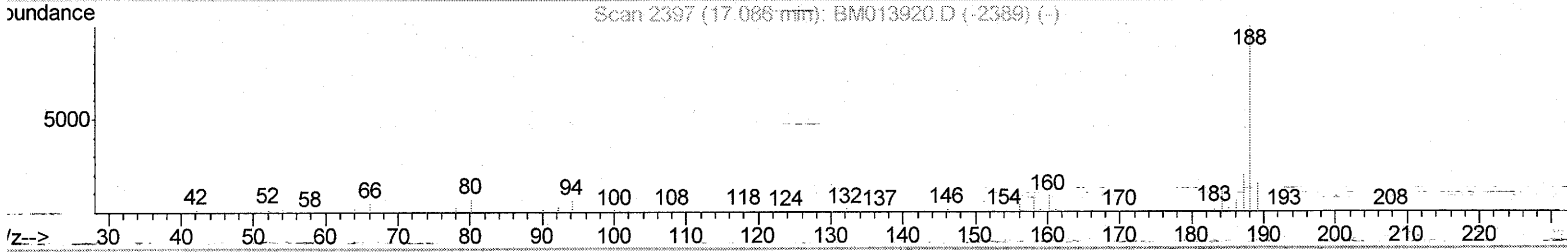
TIC: BM013910.D
