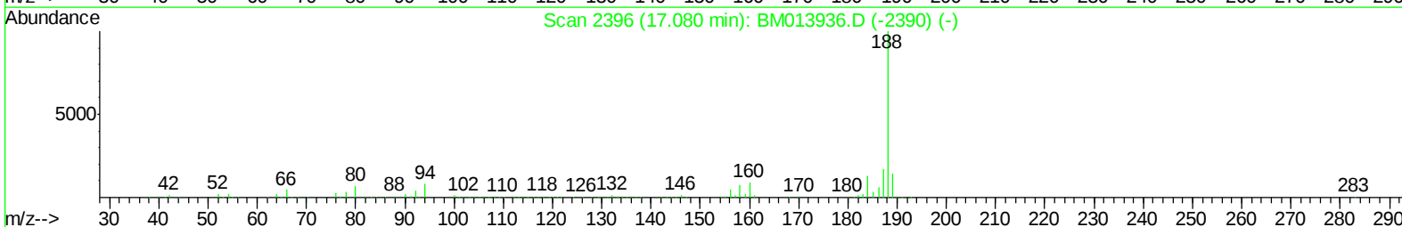
TIC: BM013945.D
