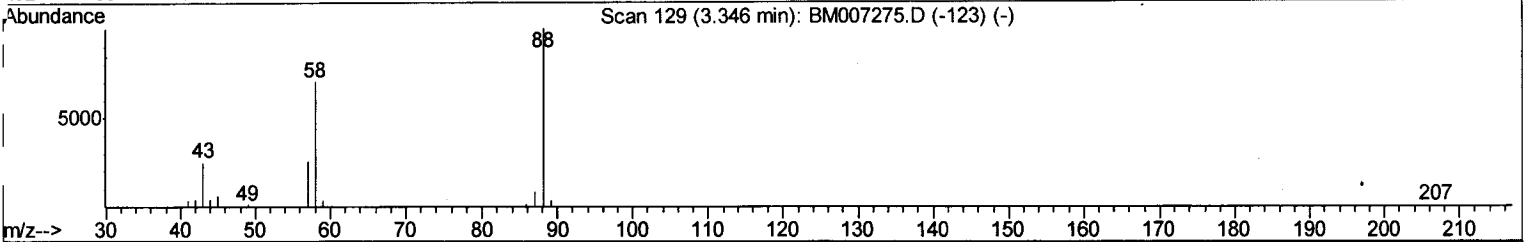
TIC: BM007276.D
