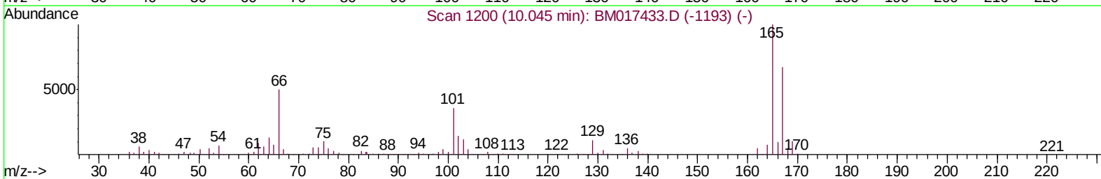
TIC: BM017439.D
