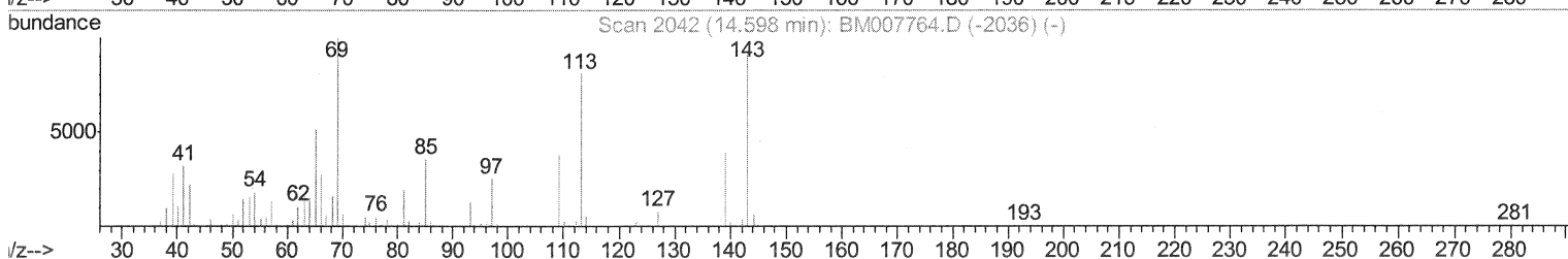
TIC: BM007812.D
