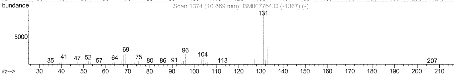
TIC: BM007812.D
