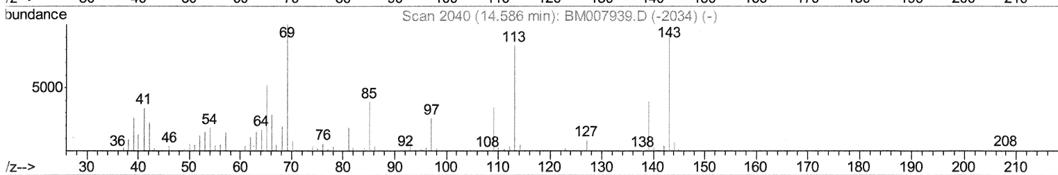
TIC: BM007944.D
