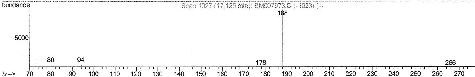
TIC: BM007966.D
