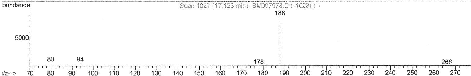
TIC: BM007982.D
