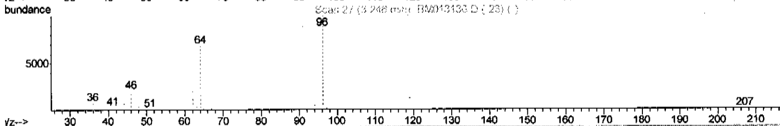
TIC: BM013139.D
