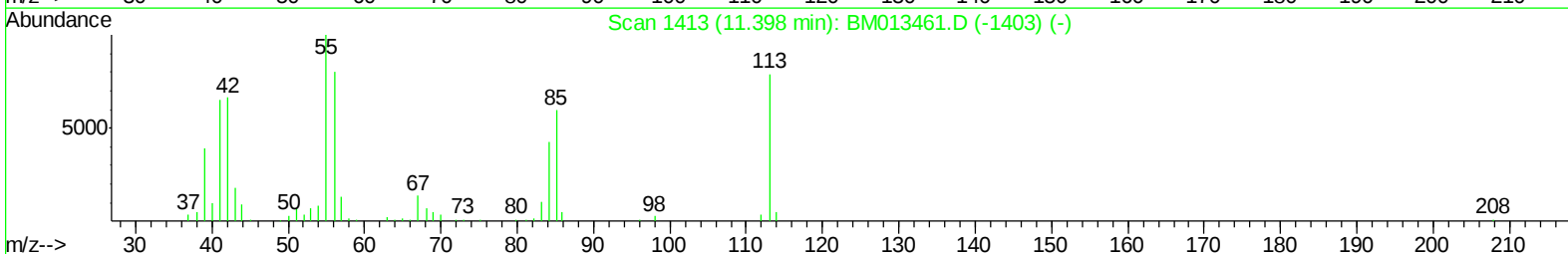
TIC: BM013477.D
