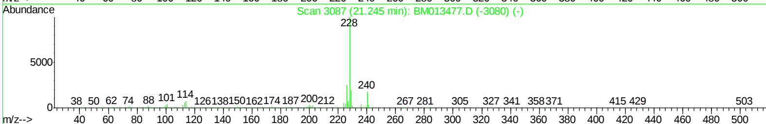
TIC: BM013481.D
