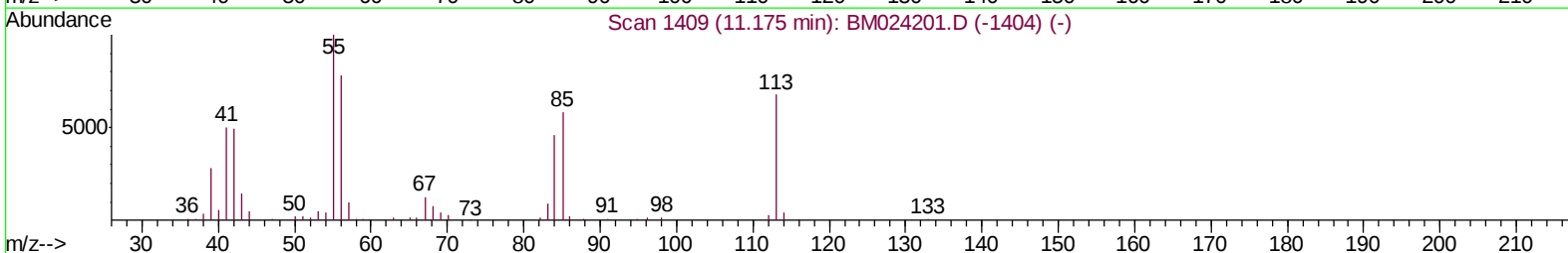
TIC: BM024203.D
