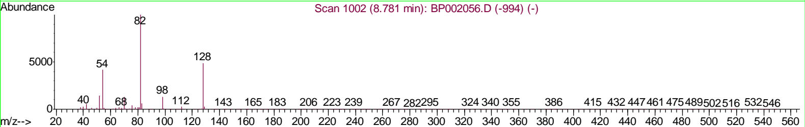
TIC: BP002063.D
