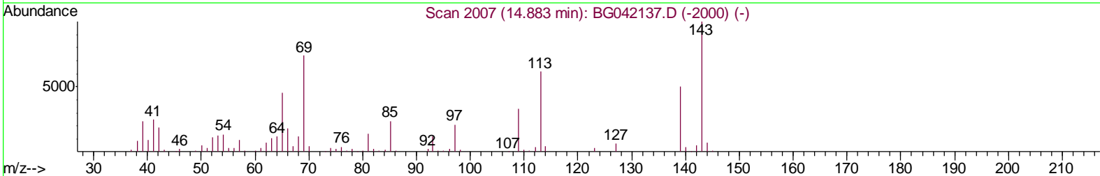
TIC: BG042139.D
