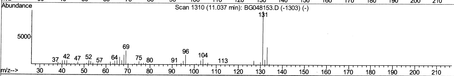
TIC: BG048162.D
