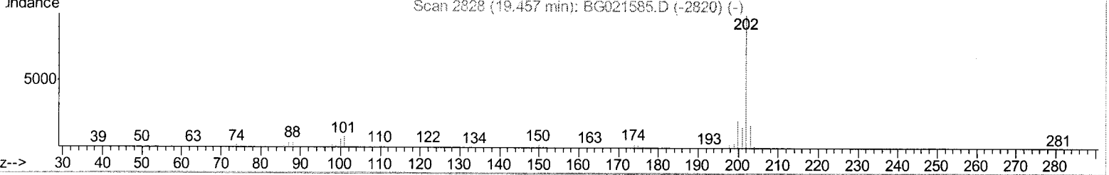
TIC: BG021585.D
