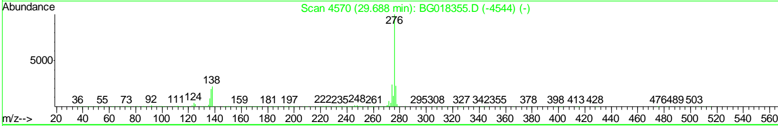
TIC: BG018369.D
