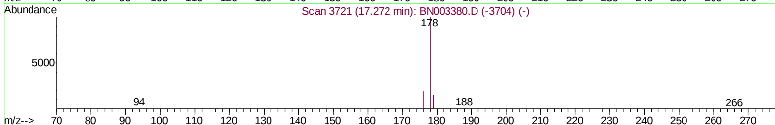
TIC: BN003390.D
