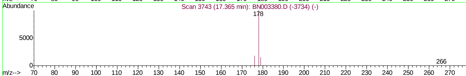
TIC: BN003392.D
