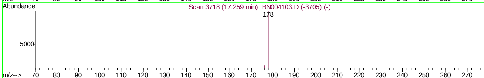
TIC: BN004109.D
