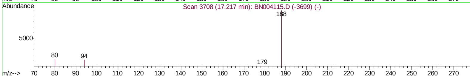
TIC: BN004122.D
