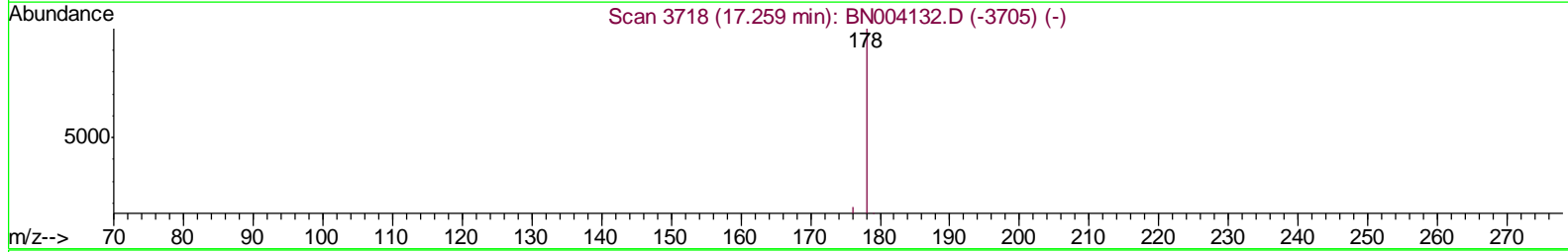
TIC: BN004139.D
