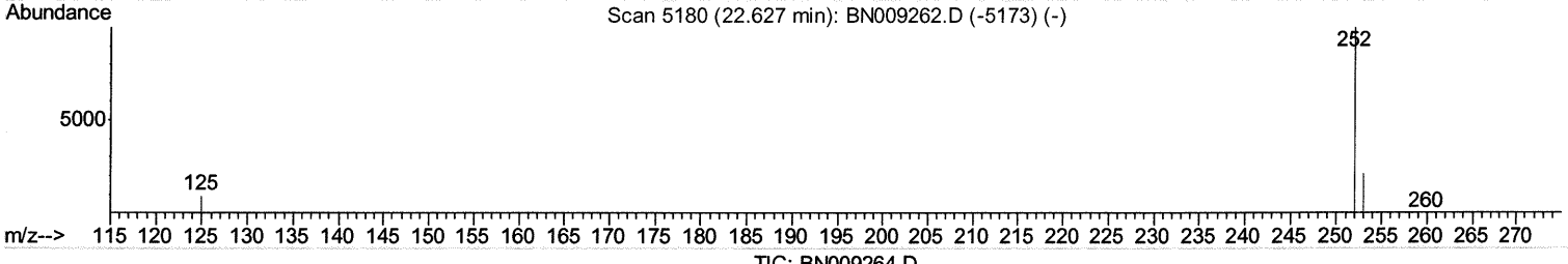
TIC: BN009264.D
