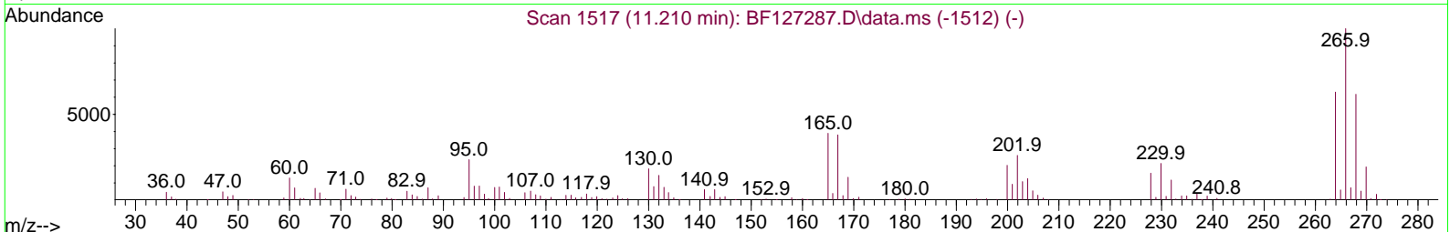
TIC: BF127294.D\data.ms
