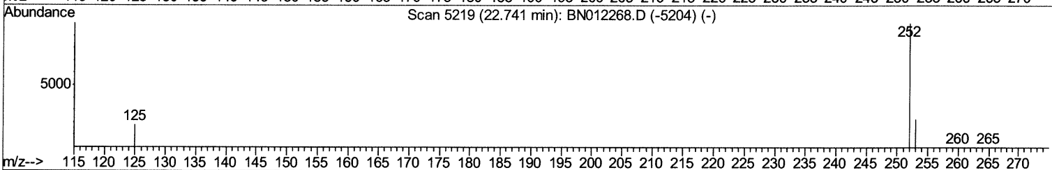
TIC: BN012280.D
