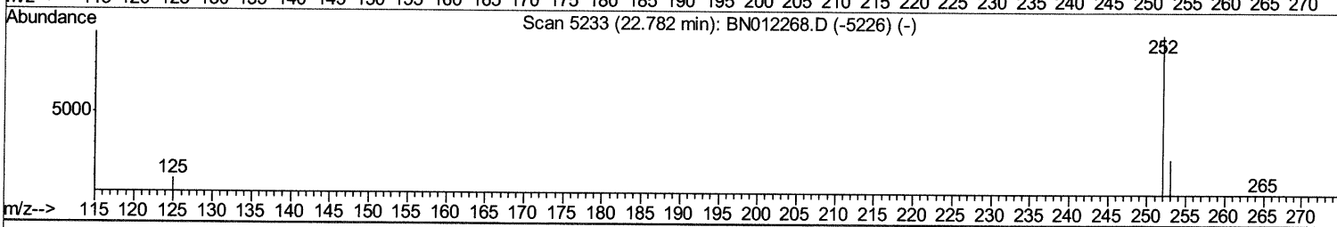
TIC: BN012280.D
