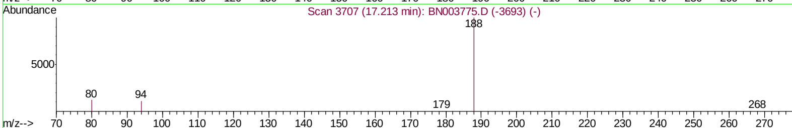
TIC: BN003783.D
