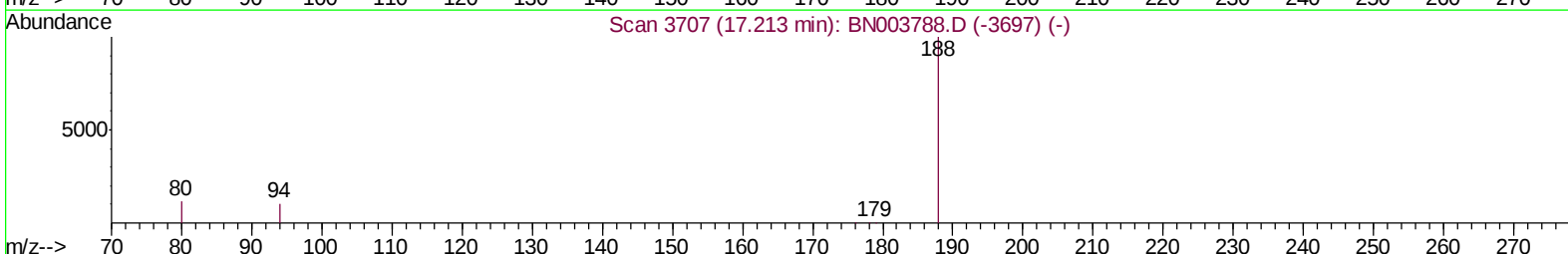
TIC: BN003797.D
