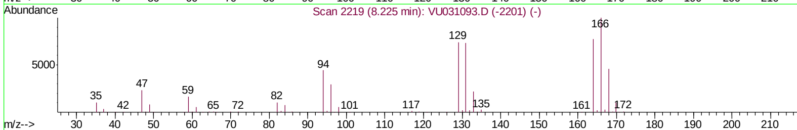
TIC: VU031120.D
