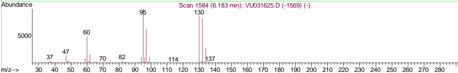
TIC: VU031626.D
