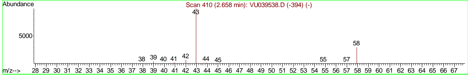
TIC: VU039557.D
