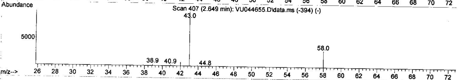
TIC: VU044675.D\data.ms
