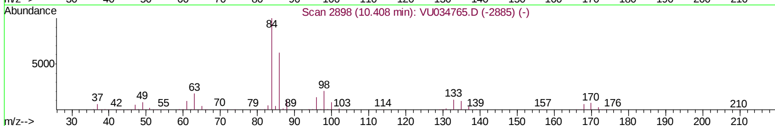
TIC: VU034778.D
