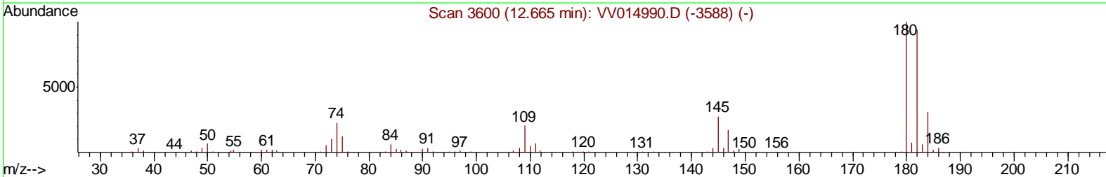
TIC: VV015009.D
