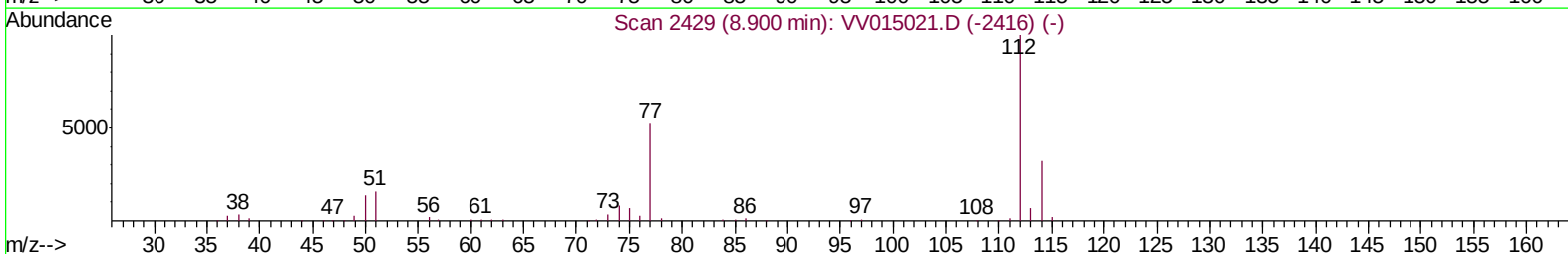
TIC: VV015037.D
