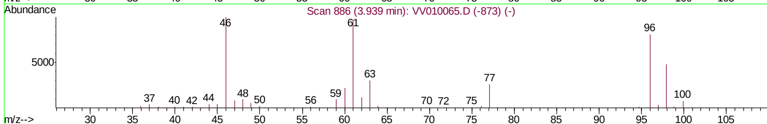
TIC: VV010069.D
