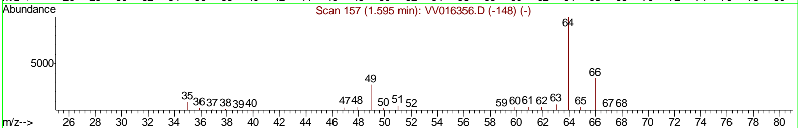
TIC: VV016363.D
