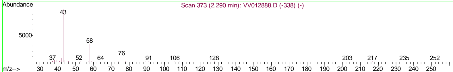
TIC: VV012895.D
