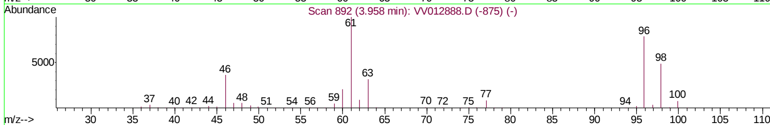
TIC: VV012904.D
