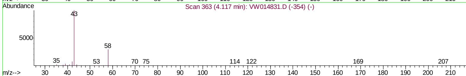
TIC: VW014835.D
