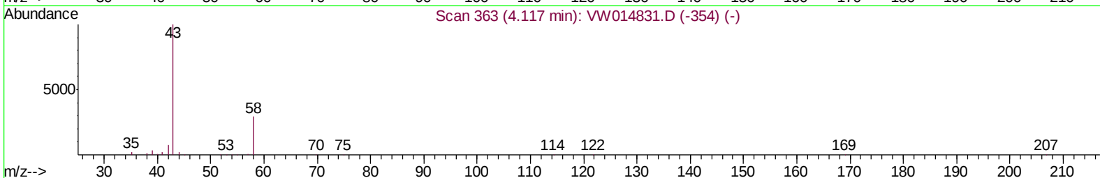
TIC: VW014847.D
