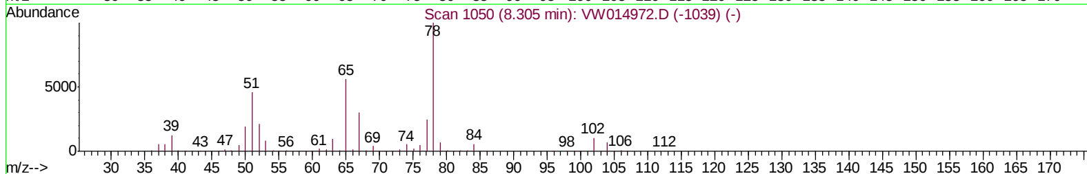
TIC: VW014979.D
